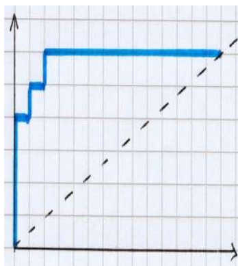
Figure 10.7: Scaling the plot's axes creates a proportionate comparison, regardless of the initial balance of positive and negative examples
