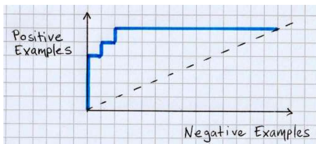
Figure 10.6: The ROC curve can be created by hand on graph paper by plotting the number of positive examples versus the number of negative examples
