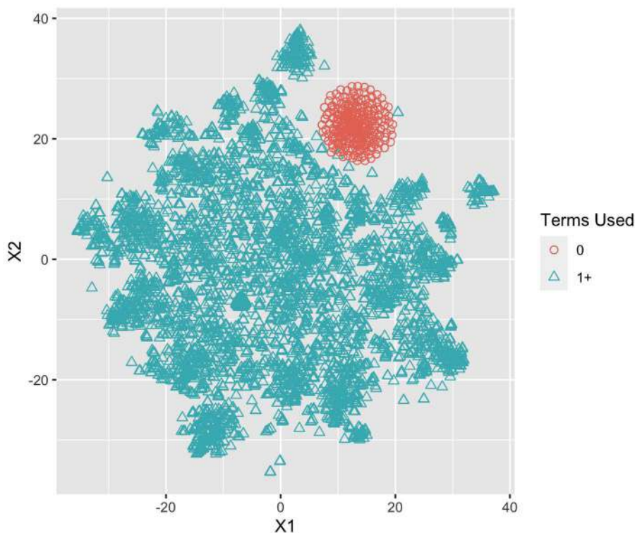
Figure 15.11: Adding color or changing the point style can help understand the clusters depicted in the t-SNE visualization
